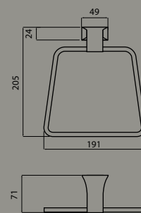
Towel Ring
