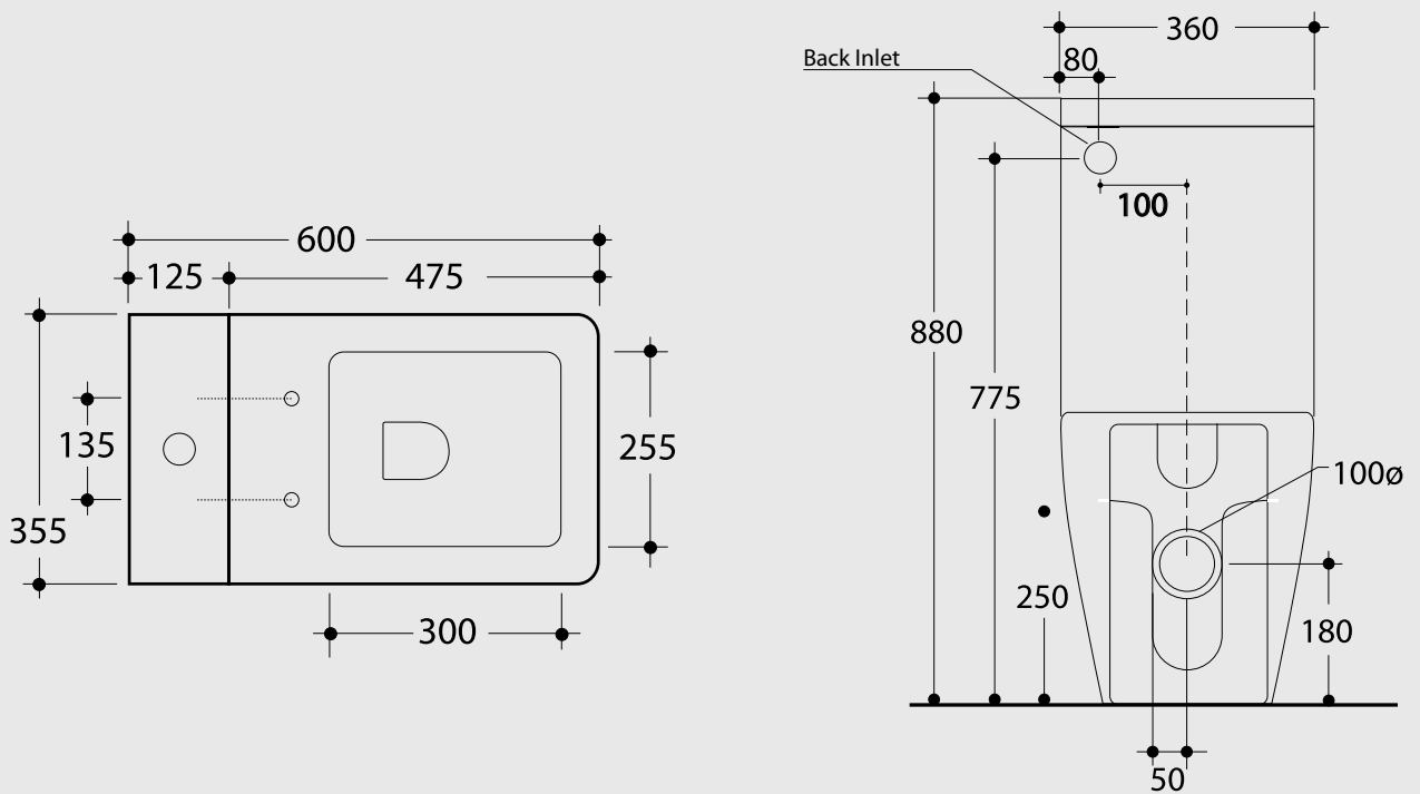
Wall faced Toilet Suite with Soft-Close Seat KER3217
